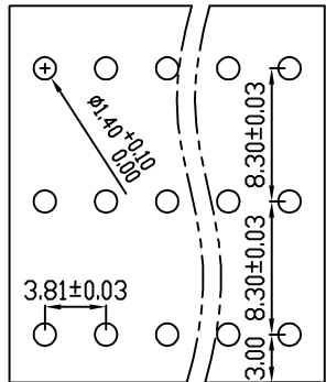
PCB LAYOUT
