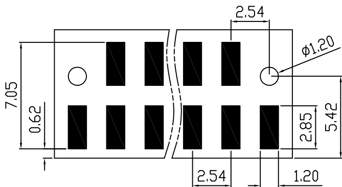
PCB Layout
